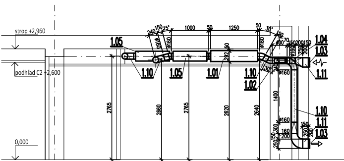
REZ A–A
